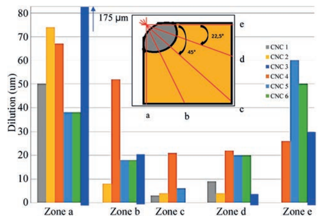
Fig. 9. Measurement of the DZ depth over the entire cross-section and DZ depth along the five red lines for all the samples
