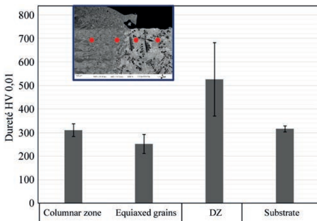
Fig. 8. Hardness measurements corresponding to the characteristic features encountered from the coating to the substrate (red points)
