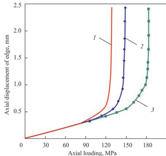
Fig re 7 Stability of cylinder shells produced by different methods to effect of axial compression loads: 1 — from solid sheet; 2 — from multilayer circle deposit; 3 — from multilayer spiral deposit
