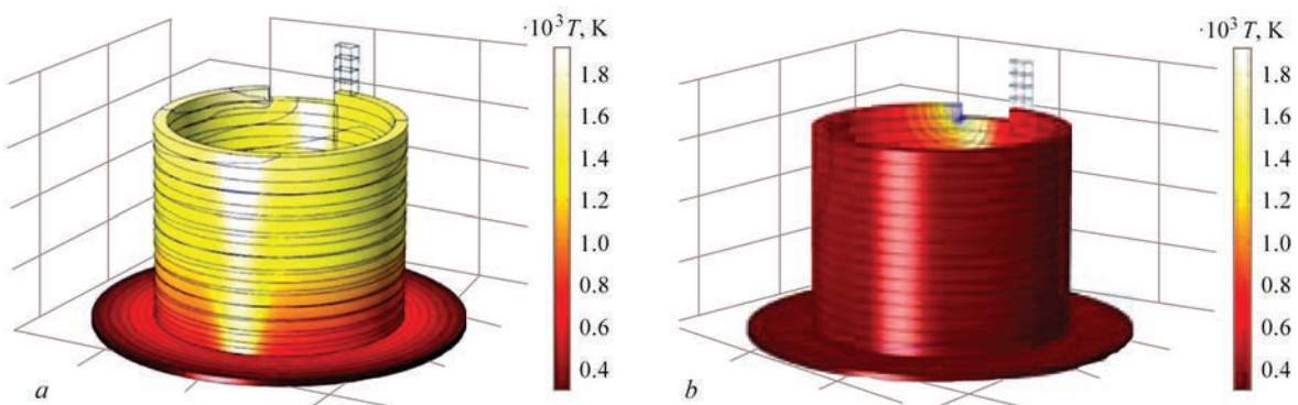
Fig re 4 Effect of deposition material on temperature field in shell: a — alloy 1561; b — Grade 2
