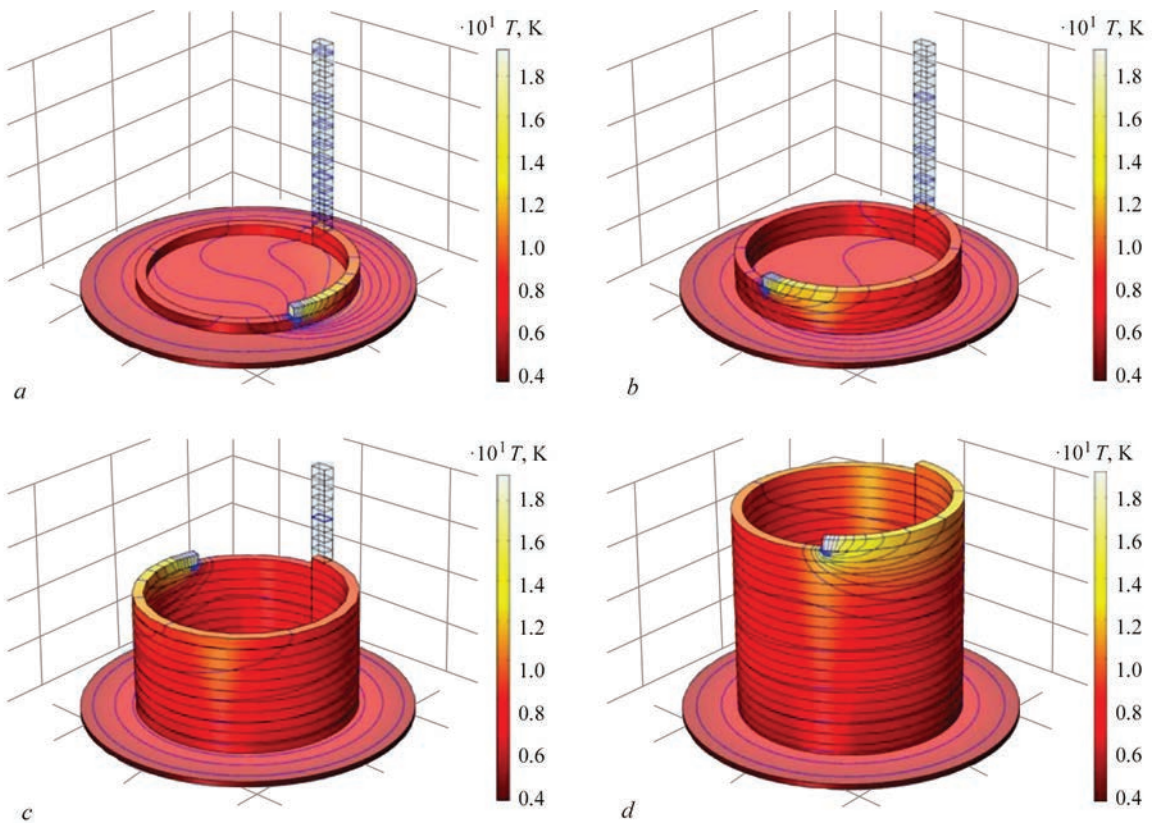
Fig re 3 Distribution of temperature in cylinder shell of titanium alloy Grade 2 obtained at 0.1 rps rate by time: a — 13; b — 35; c — 108; d — 194 s
