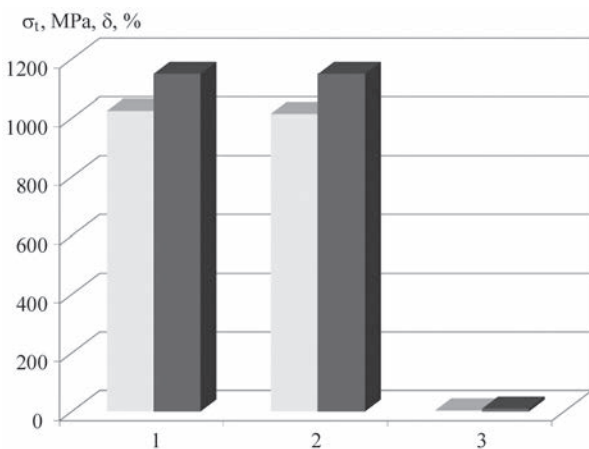
Figure 5. Comparative results of mechanical testing of samples of TC4 titanium alloy (light grey colour) welded by laser-microplasma method and base metal (dark-grey colour) at their static tension: 1, 2 — averaged ultimate strength \sigma_t (MPa) for samples of 1.0 (1) and 3.0 (2) mm thickness; 3 — relative elongation \delta (%) for all the cases
